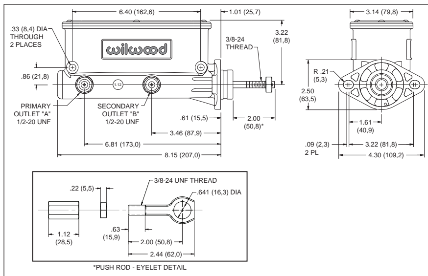
Wilwood Dual Outlet Tandem Chamber Master Cylinder, Mounting Dimensions
