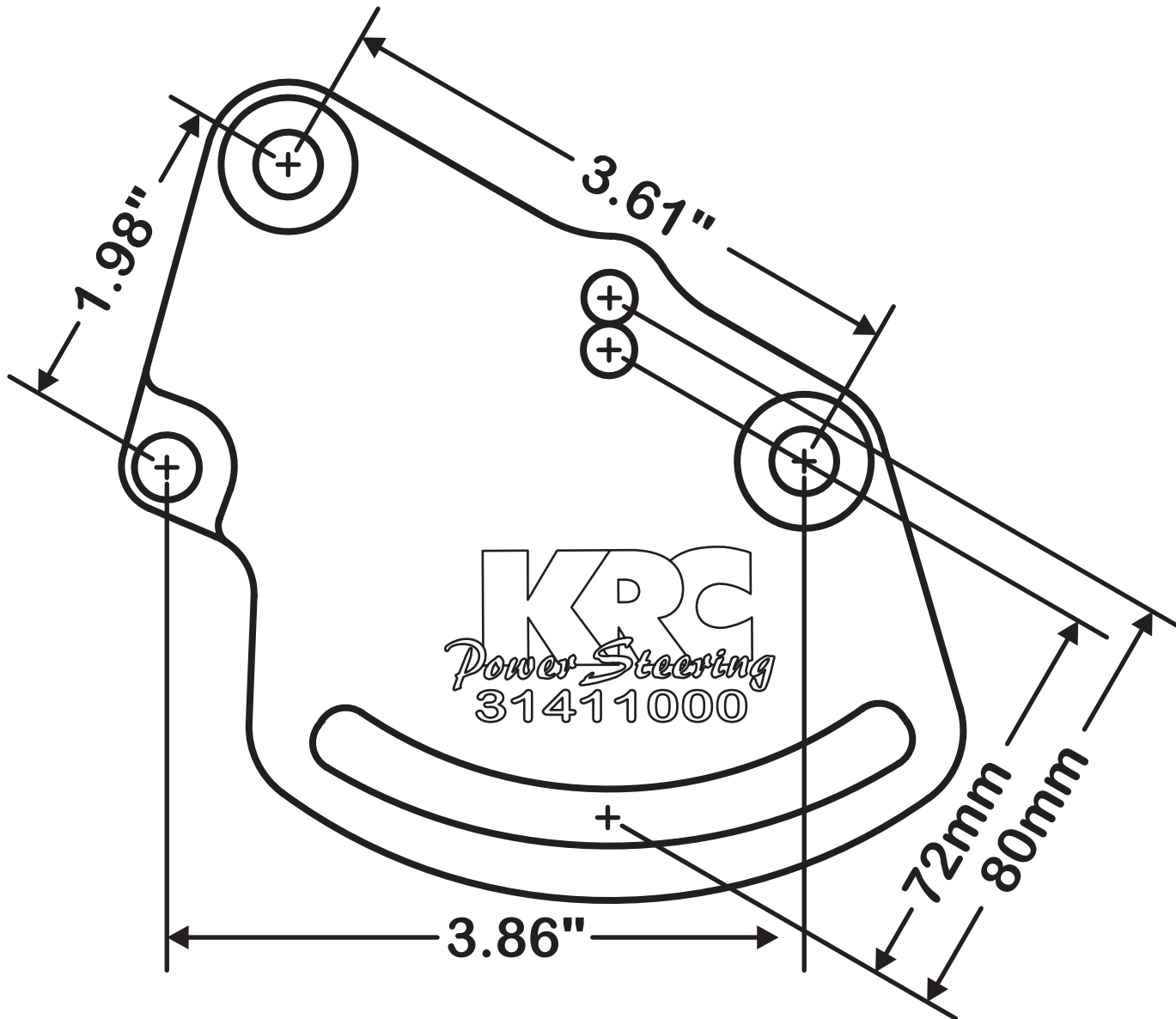
Small Block Chevrolet Left Head
