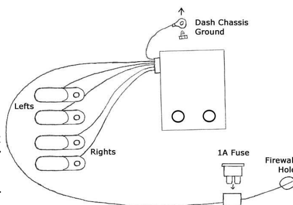
Drawing 1: Wiring Diagram
