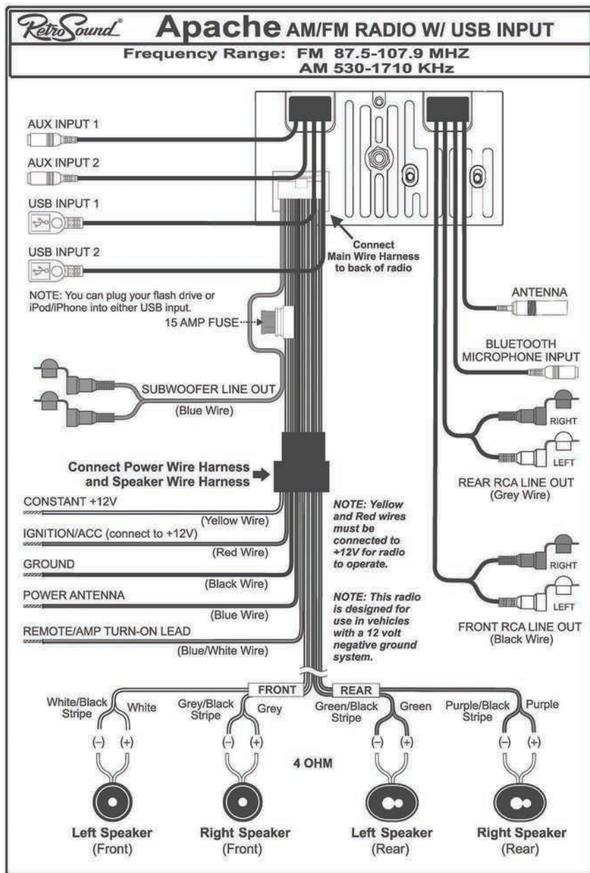
Figure 9 - Wiring Diagram
