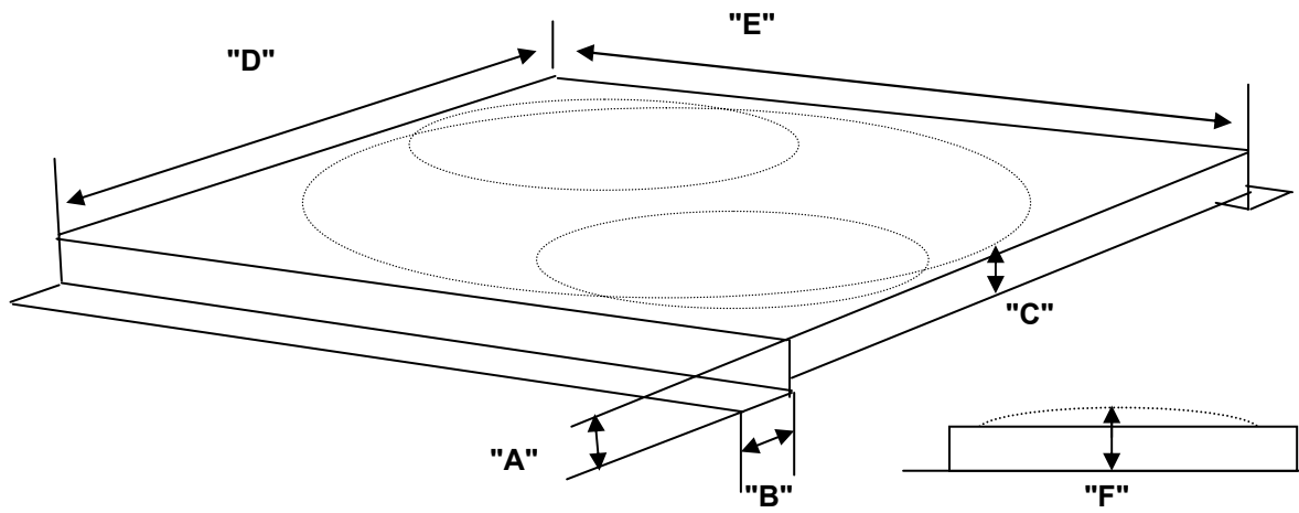
Fan Shroud Measurements
