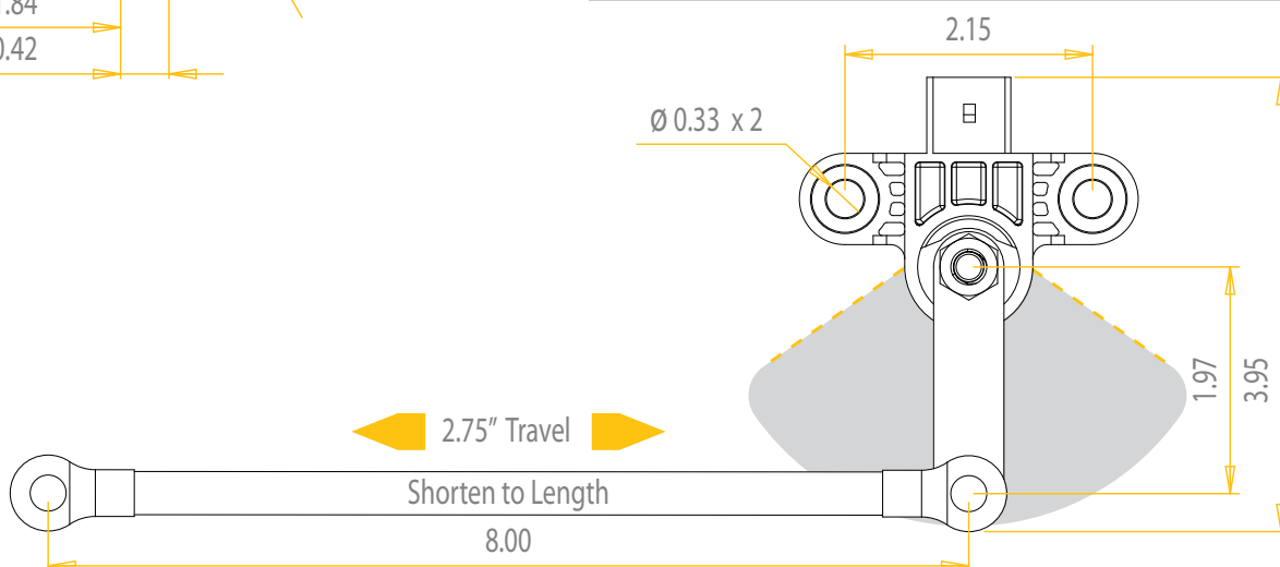
Dimensions In Inches (Not To Scale)
