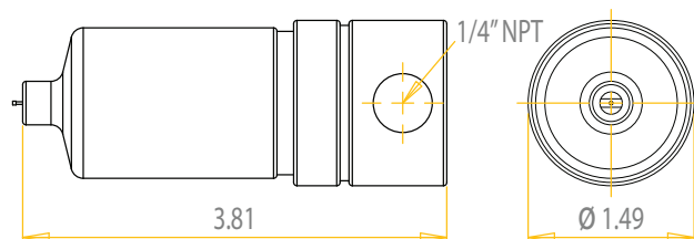
Dimensions In Inches (Not To Scale)
