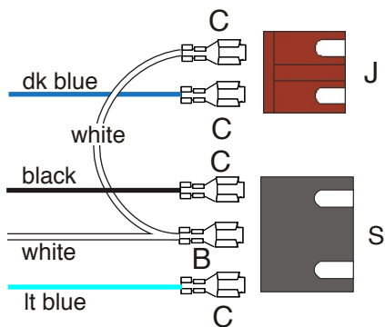
64-65 2 Speed with washer
