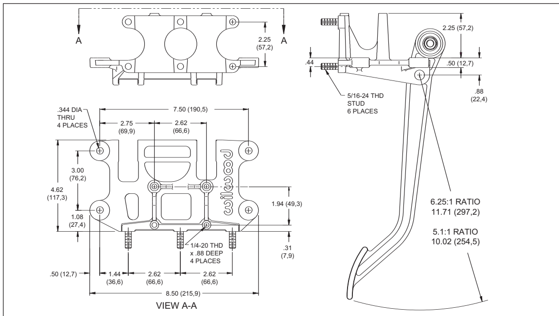
Reverse Mount Dual Pedal Assembly, Physical Dimensions (applicable to both part numbers)
