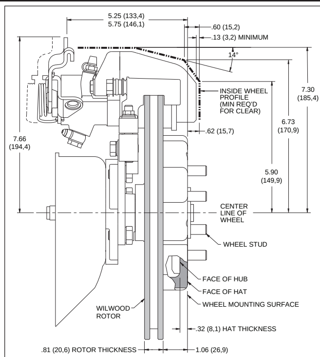
Figure 2. Wheel Clearance Diagram
