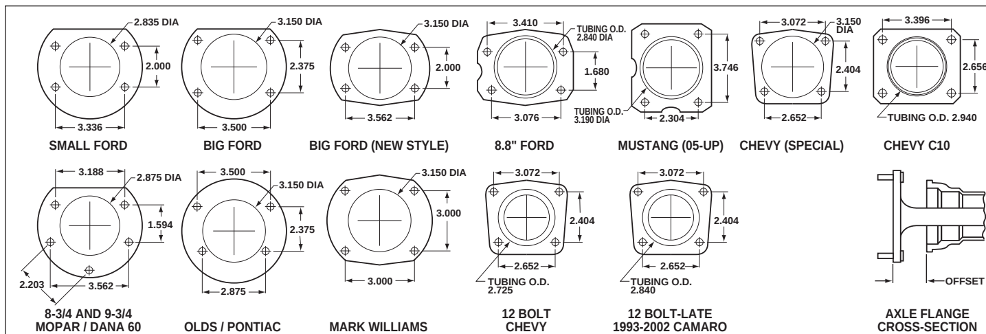
Figure 4. Rear Housing Flange Chart and Axle Flange / Offset Cross-Section
