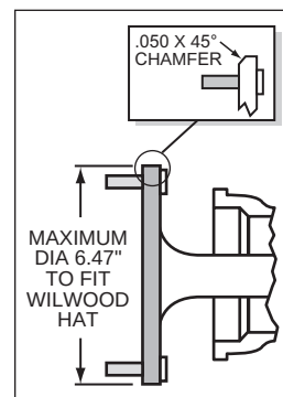
Figure 3. Axle Flange Maximum Dimension
