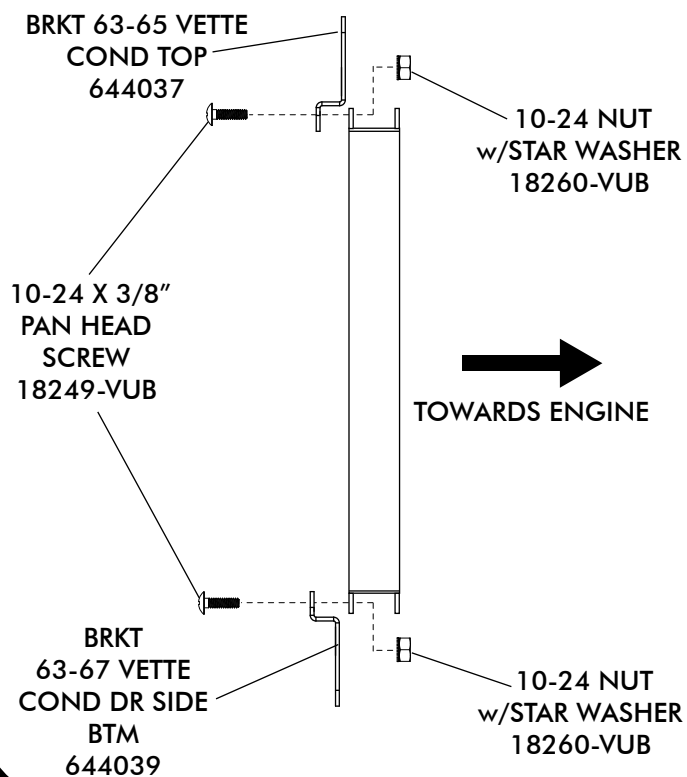
SIDE VIEW OF CONDENSER
