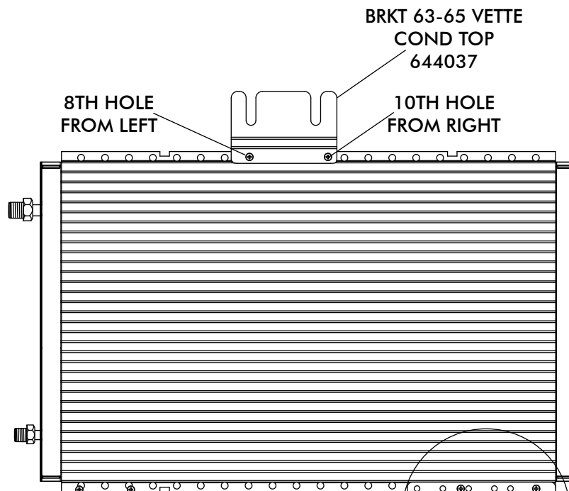
SIDE VIEW OF CONDENSER
