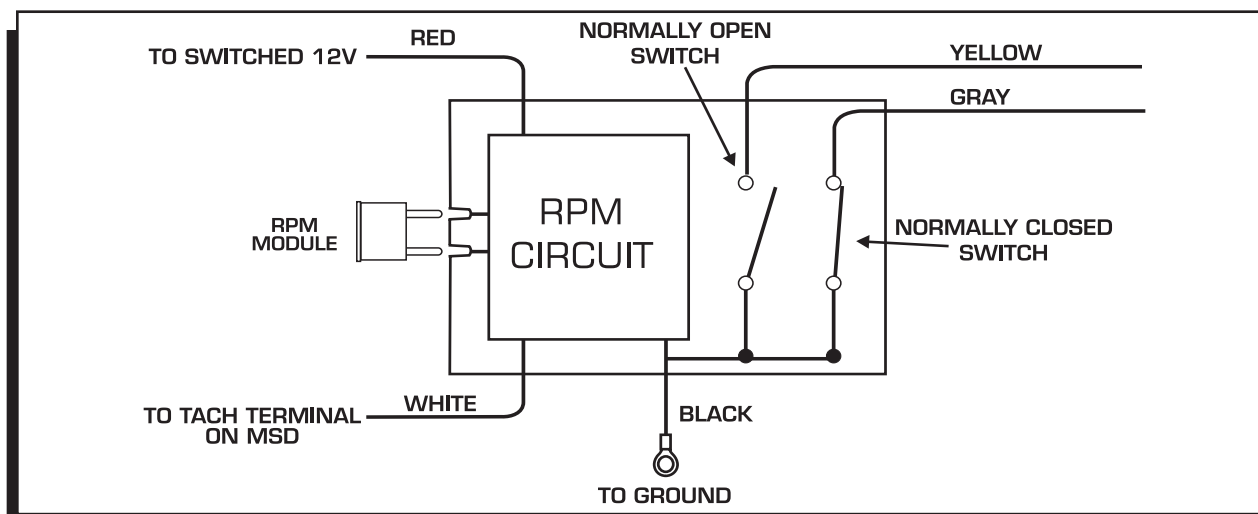
Figure 1 Operation of the RPM Activated Switch.
