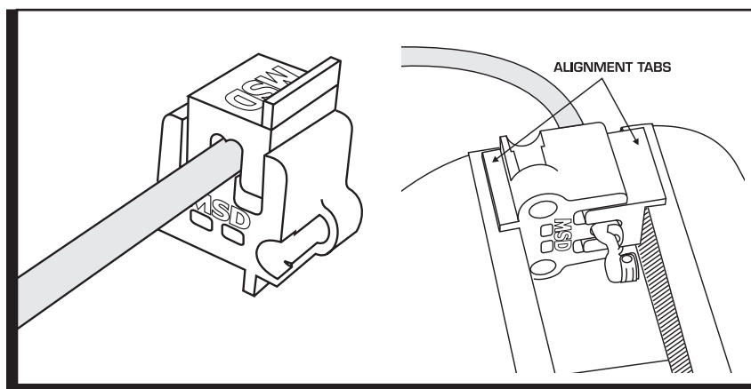
Figure 10 Crimping the Terminal.
