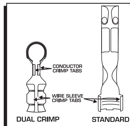
Figure 5 Identifying the Different Style Terminals.
