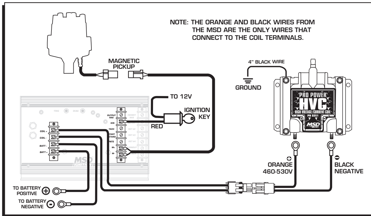
Wiring to an MSD 7AL-3
