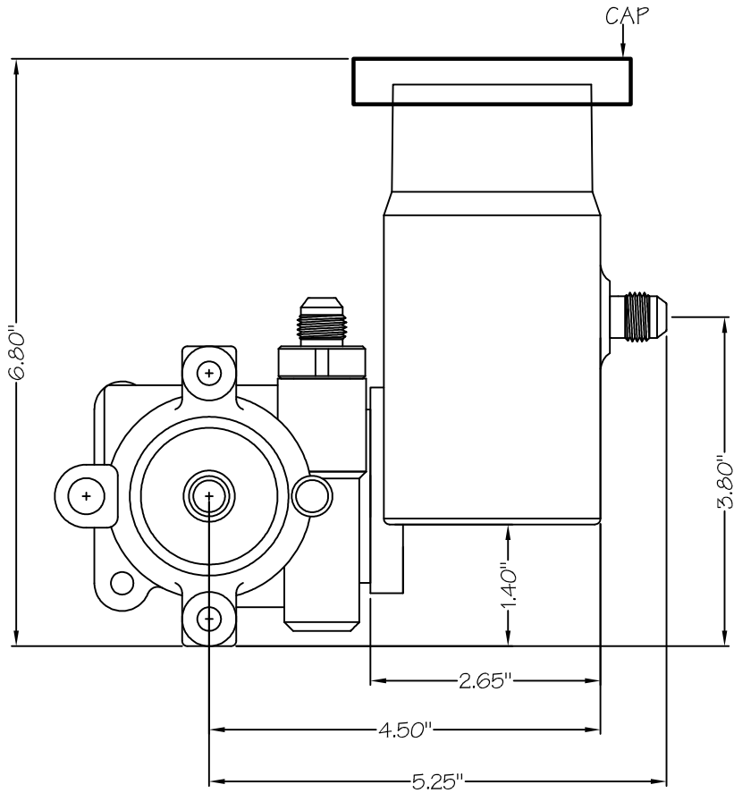
Aluminum Pump with Tank Front View
