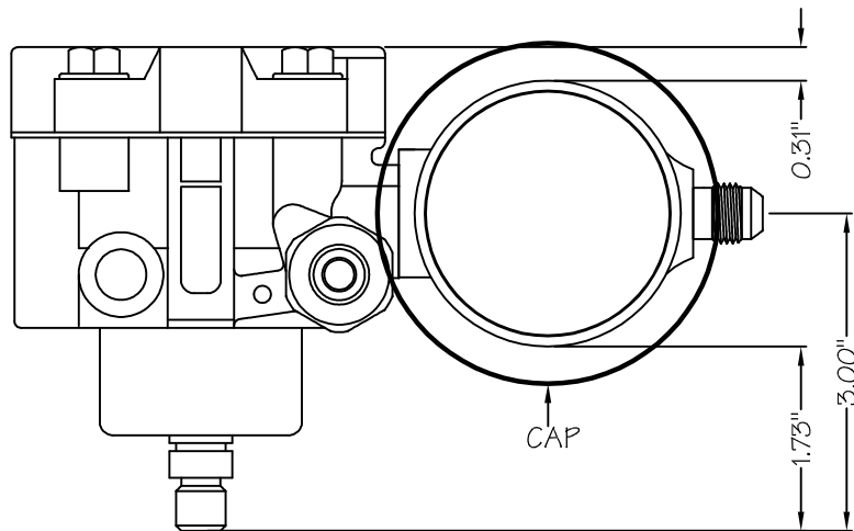
Aluminum Pump with Tank Top View
