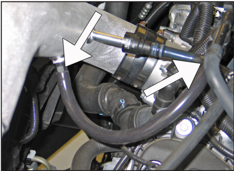
21. Install the provided silicone hose onto the 3/8" hose fitting installed in the K&N® intake tube; attach the open end to the EVAP check valve.
