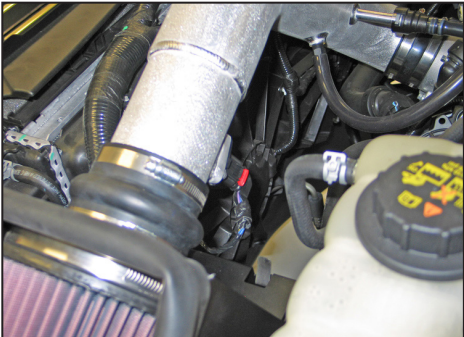
22. Reconnect the mass air sensor electrical connection.
