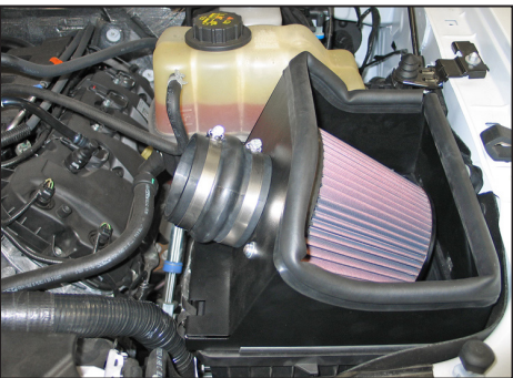
15. Install the provided silicone hose (5-576) onto the filter adapter and secure with the provided hose clamp.
