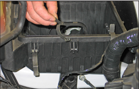
12. Remove the center airbox retaining clip.
