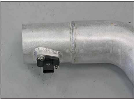
18. Install the mass air sensor into the K&N® intake tube and secure with the provided hardware.
