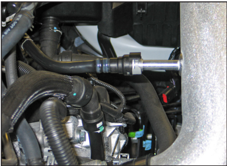
20. Connect the crankcase vent hose to the quick disconnect fitting on the K&N® intake tube. NOTE: It is necessary to rotate the plastic crank case vent tube on the plastic connector that attaches to the valve cover approximately ¼ turn counter clockwise for the tube to align with the fitting on the K&N® intake tube.
