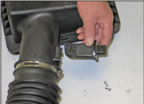
17. Remove the two screws securing the mass air sensor, then remove from the stock intake tube as shown.
