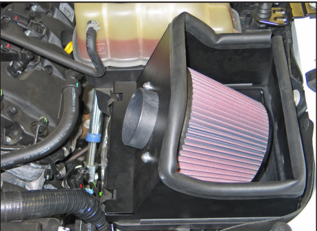
13. Install the heat shield/filter assembly onto the lower airbox and secure with the factory airbox retaining clips. NOTE: A small gap may be visible between the heat shield and lower airbox. NOTE: Drycharger® air filter wrap; part # RC-5173DK is available to purchase separately. To learn more about Drycharger® filter wraps or look up color availability please visit http://www.knfilters.com® .
