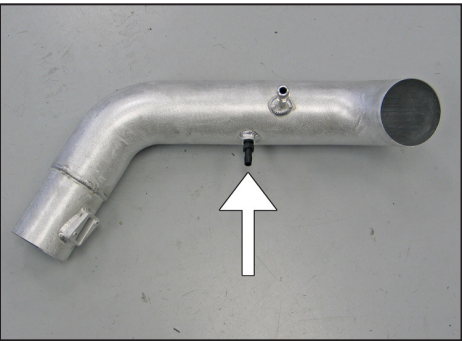
16. Install the provided 3/8" hose fitting into the K&N® intake tube as shown. NOTE: Plastic NPT fittings are easy to cross thread. Install the vent fitting "hand" tight, then turn it two complete turns with a wrench.
