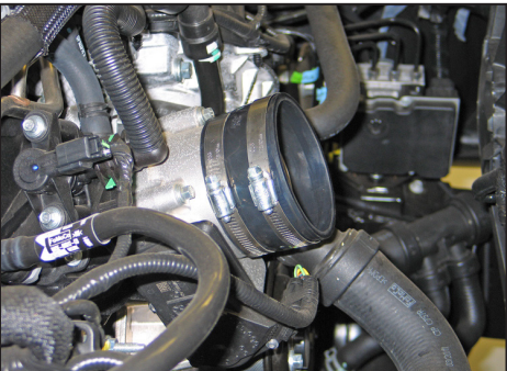
14. Install the provided silicone hose (08630) onto the throttle body and secure with the provided hose clamp.
