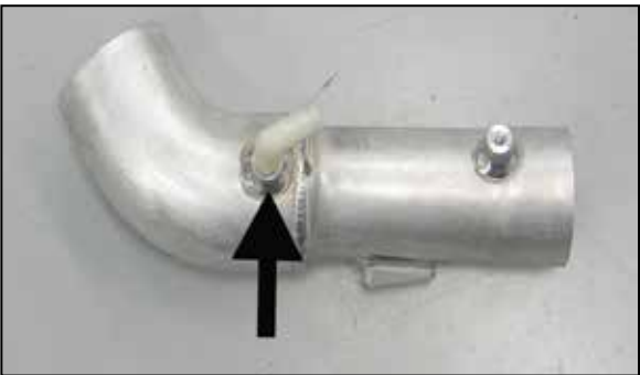
19. Install the provided 90°npt vent fitting into the driver's side K&N® intake tube (27466) as shown. NOTE: Plastic NPT fittings are easy to cross thread. Install the vent fitting "hand" tight, then turn it two complete turns with a wrench.
