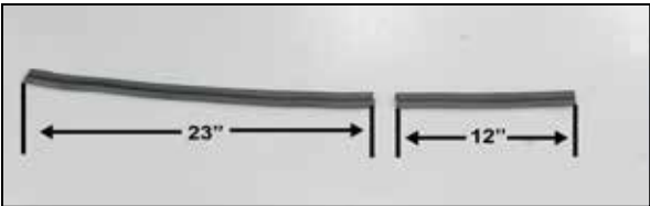
16. Cut the provided edge trim into two sections as shown, one section will be 12" long and the other section should be 23" long as shown.
