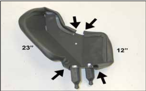
17. Install the trimmed edge trim onto the heat shield as shown. NOTE: Be sure to leave a gap for the tube mounting bracket as shown.
