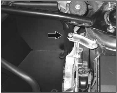
16. Place the supplied spacer under the heat shield mounting bracket and then secure the bracket to the ECU mounting bracket with the provided hardware as shown.
