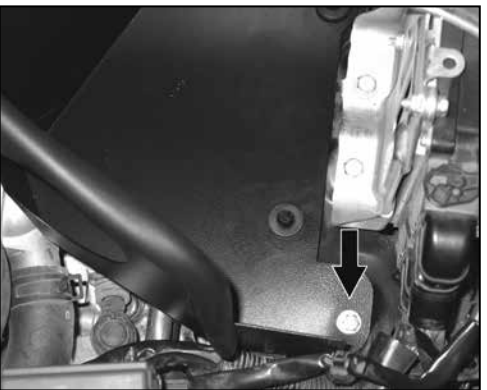
17. Secure the front of the heat shield to the front air box mount with the provided hardware. Tighten all the heat shield mounting bolts.
