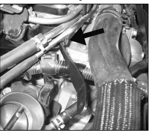
18b. Secure the provided tube mounting bracket (083140) to the engine using the provided hardware. NOTE: Be sure to resecure the vacuum lines under the tube mounting bracket.
