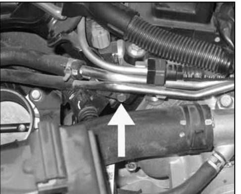
18a. On vehicles not equipped with an EGR tube, remove the bolt shown which secures the steel vacuum lines to the engine.
