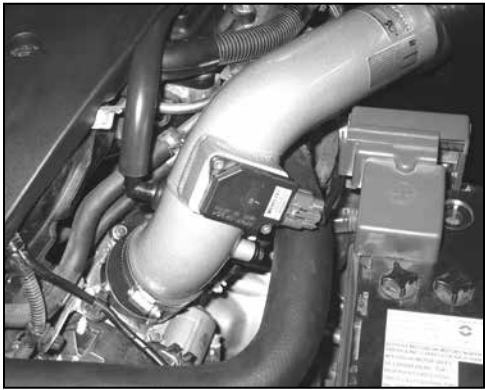
27. Reconnect the mass air sensor electrical connection.
