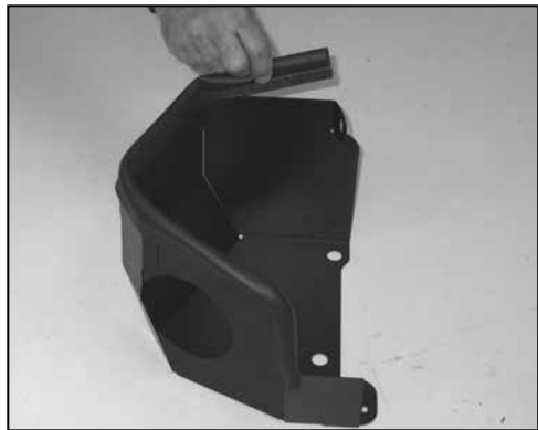
11. Install the long piece of the edge trim onto the heat shield as shown. NOTE: Some trimming of the edge trim may be needed.
