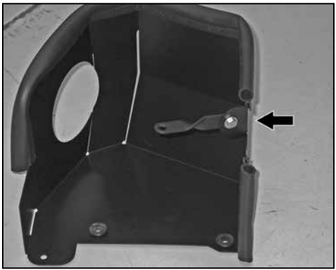
14. Install the heat shield bracket (070702) onto the heat shield as shown. NOTE: Do not completely tighten the bracket at this time.
