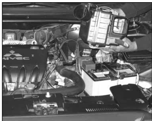
9. Lift up the air box assembly to unhook it from the mounting grommets and then remove the air box from the vehicle as shown.
