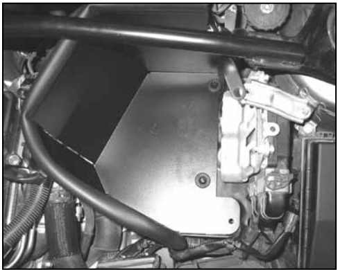
15. Install the heat shield assembly into the vehicle so that the grommets fit tightly over the factory air box mounting studs.
