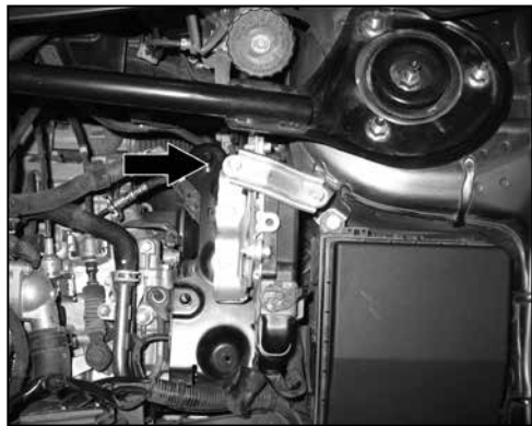
10. Remove the ECU bracket mounting bolt shown.
