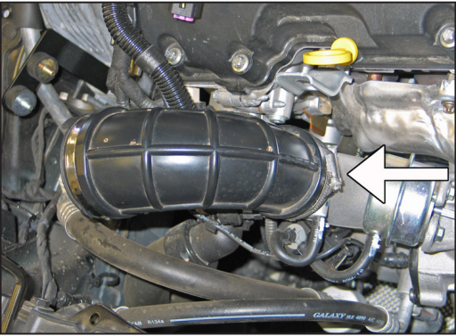
15. Loosen the hose clamp securing the intake elbow to the throttle body so that the intake elbow position can be adjusted.
