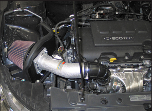
19. Reconnect the vehicle's negative battery cable. Double check to make sure everything is tight and properly positioned before starting the vehicle.
