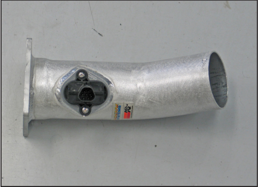
11. Install the mass air sensor into the K&N® intake tube and secure with the provided hardware.
