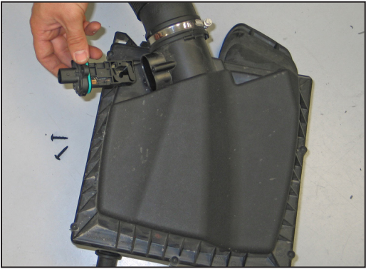
10. Remove the two screws that secure the mass air sensor to the factory airbox and then remove the mass air sensor from the airbox.
