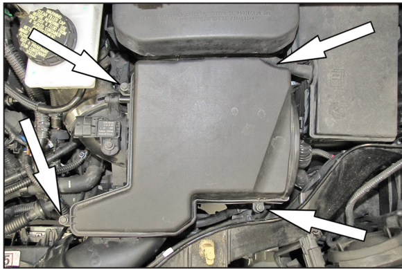
5. Loosen the four screws that secure the air filter housing lid and then remove the lid and factory air filter.
