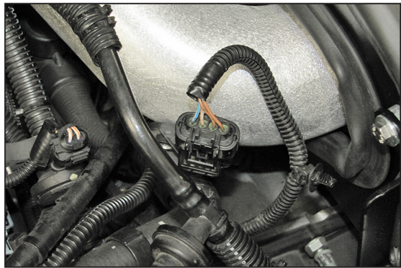
23. Reconnect the inlet air temperature sensor electrical connection.
