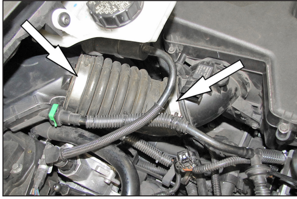
6. Loosen the two hose clamps that secure the factory intake hose.
