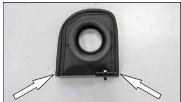
10. Install the provided edge trim onto the heat shield as shown. NOTE: Some trimming of the edge trim will be necessary.
