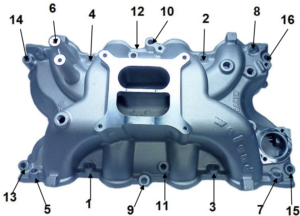
Figure 1 Bolt tightening sequence
