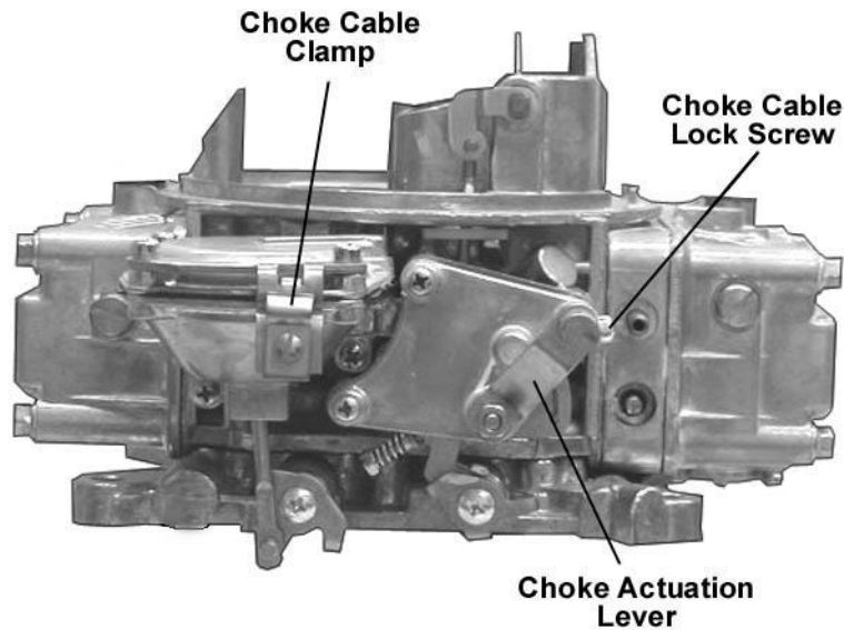
Figure 2b. Manual choke parts (0-1850 shown)
