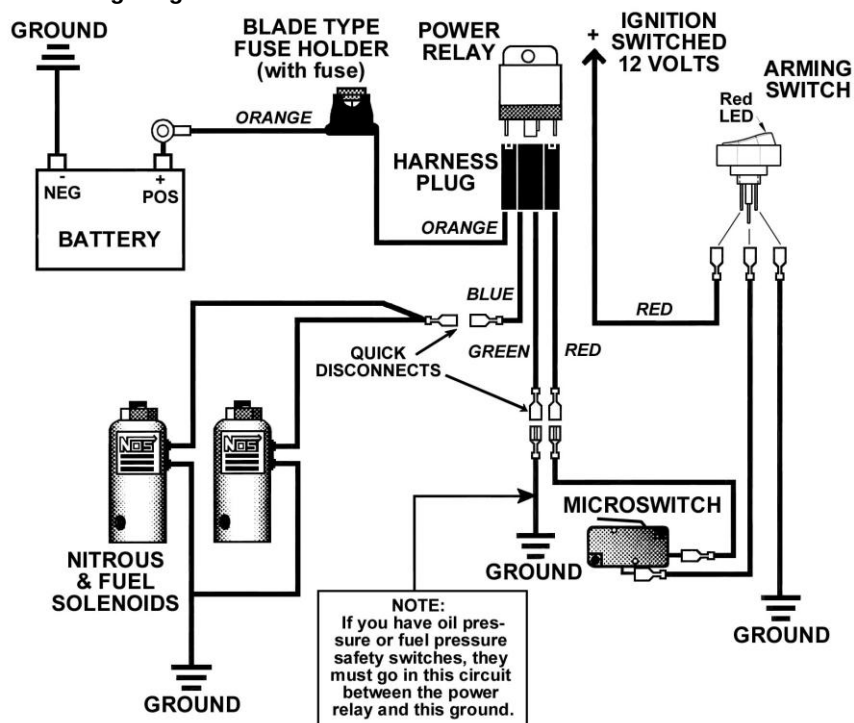
Figure 16 General Electric Wiring Diagram
