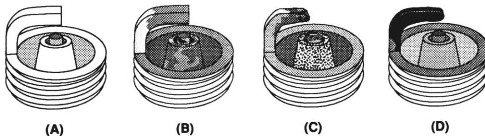
Figure 17 Spark Plug Condition
