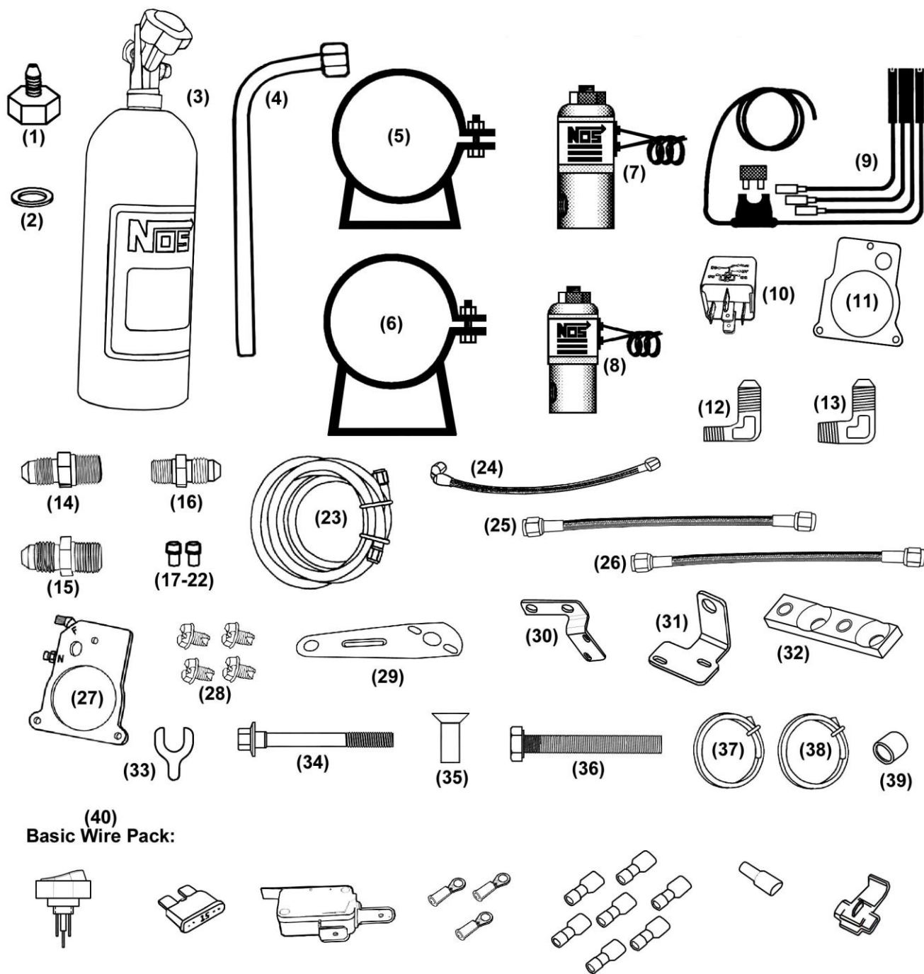
Figure 1 Kit Number 05168NOS Component Identification
