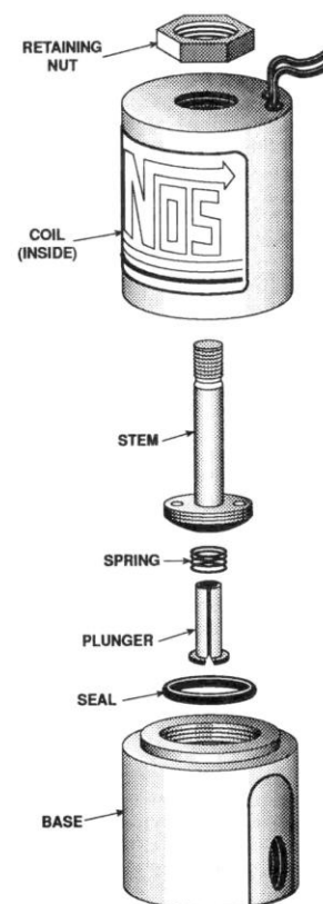
Exploded View of a Typical Solenoid
