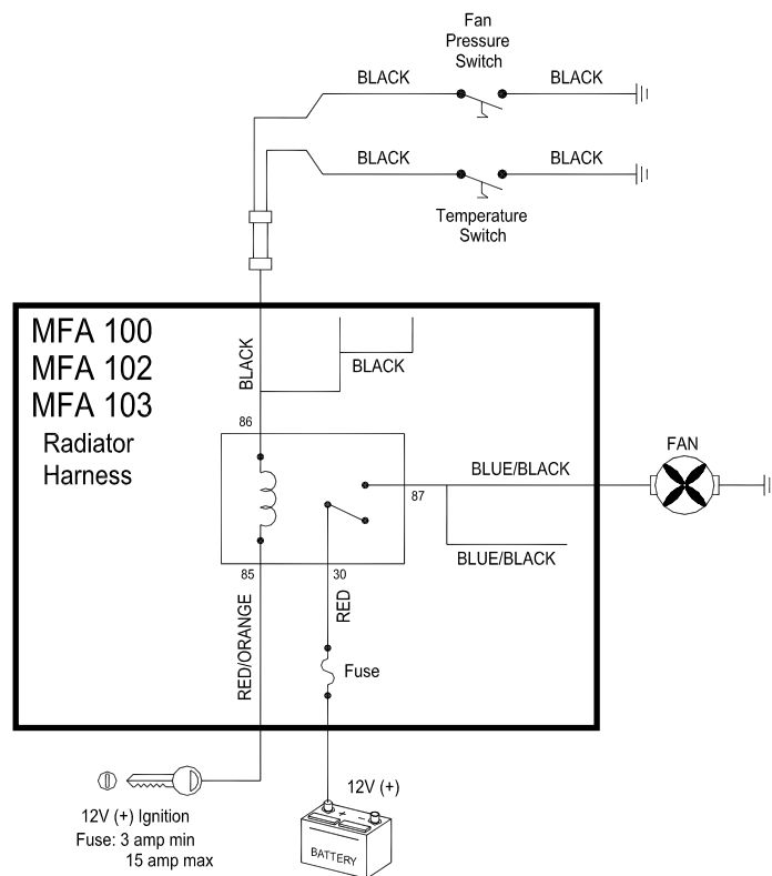
Radiator Fan with A/C with Fan Pressure Switch.
