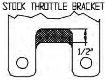
Figure 1 - Throttle Bracket Modification Remove material in the shaded area on stock throttle brackets to clear the intake manifold.
