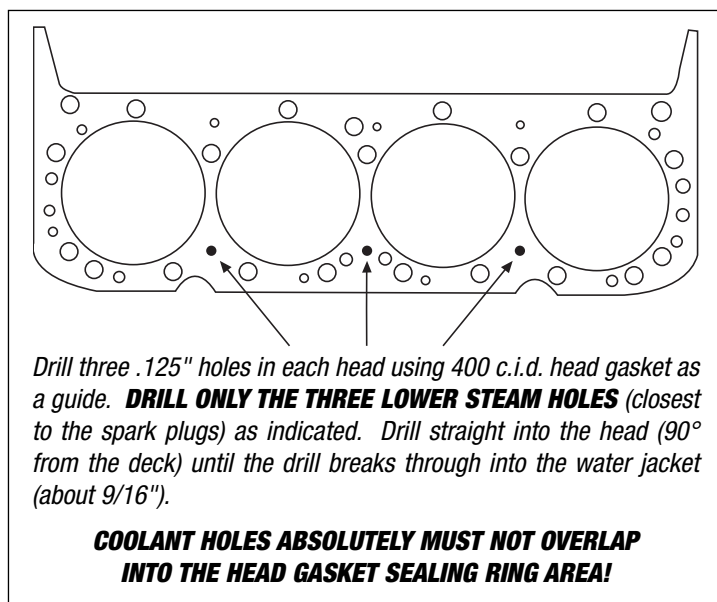
Figure 1 - Steam Hole Locations (400 C.I.D. Engines ONLY)
