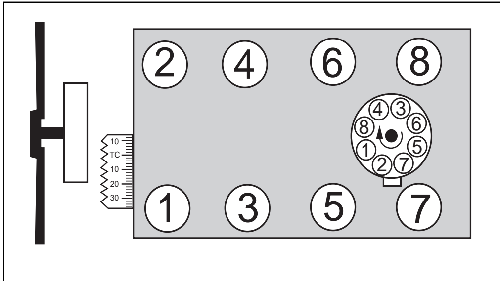
Figure 1- Chrysler 318-360 c.i.d. V8 Firing Order 1-8-4-3-6-5-7-2 Turn distributor counter-clockwise to advance timing.
