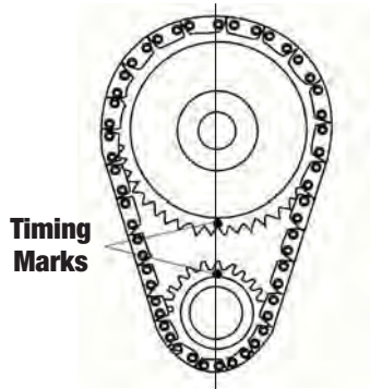
Figure 1 Timing Chain Sprocket Alignment Timing Marks
