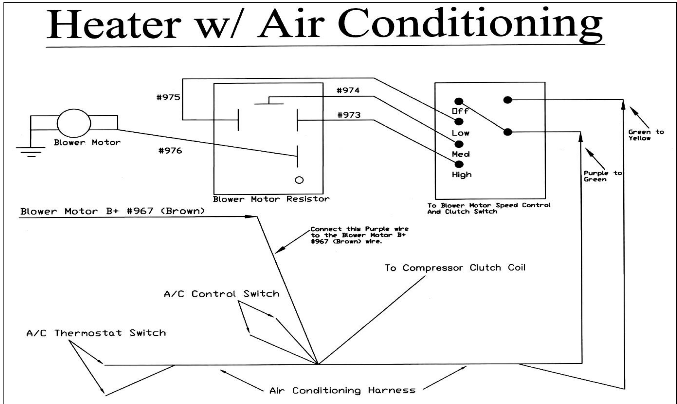
Figure 7-20 Heater with Air Conditioning
