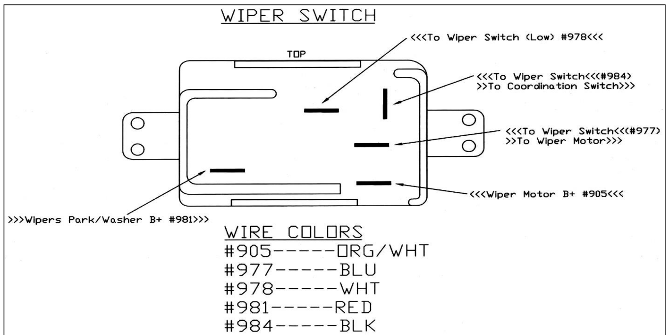
Figure 7-21 Wiper Switch Connections
