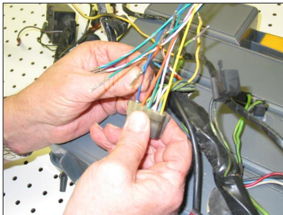
Figure 7-14 '68 Adaptor Pigtail Wires
