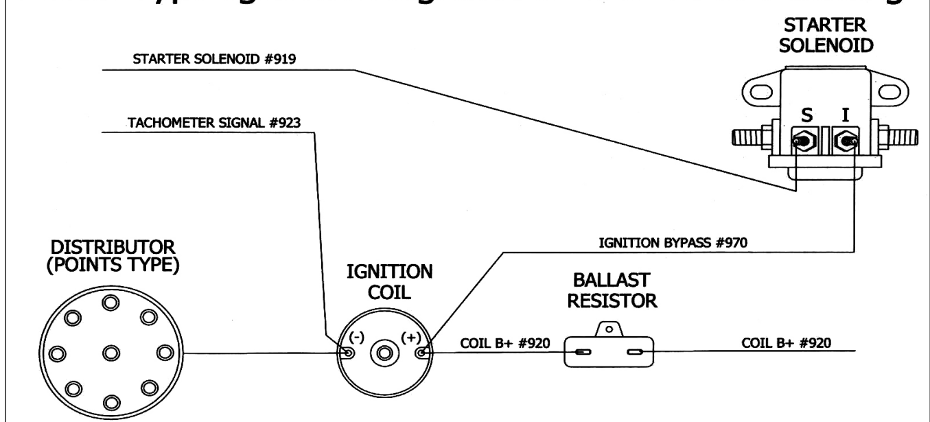
Figure 7-5 Points Type Ignition Diagram
