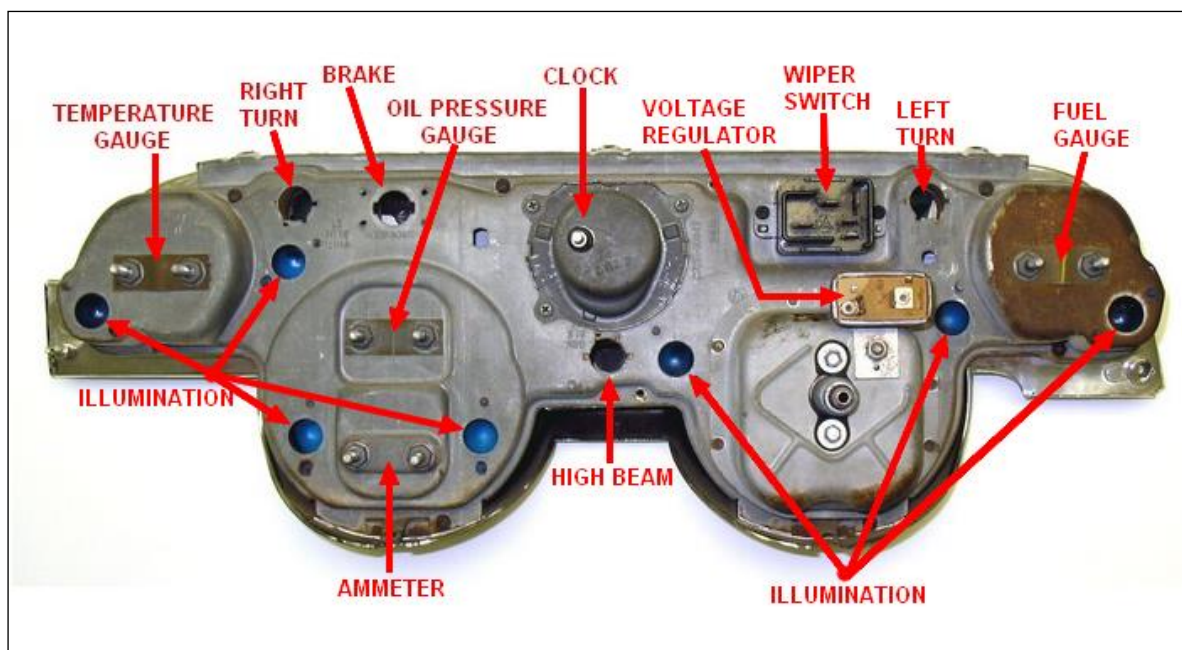
Figure 7-18 Gauge Cluster 1967 Mustang
