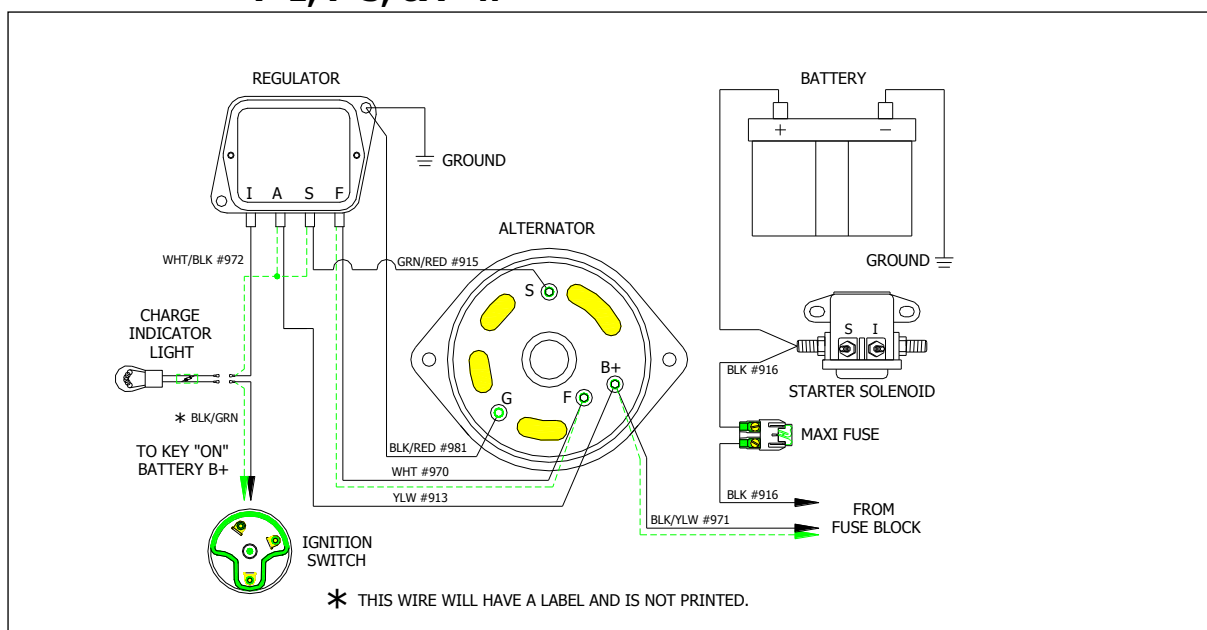
Figure 7-1 Alternator/Regulator/Solenoid Connections
