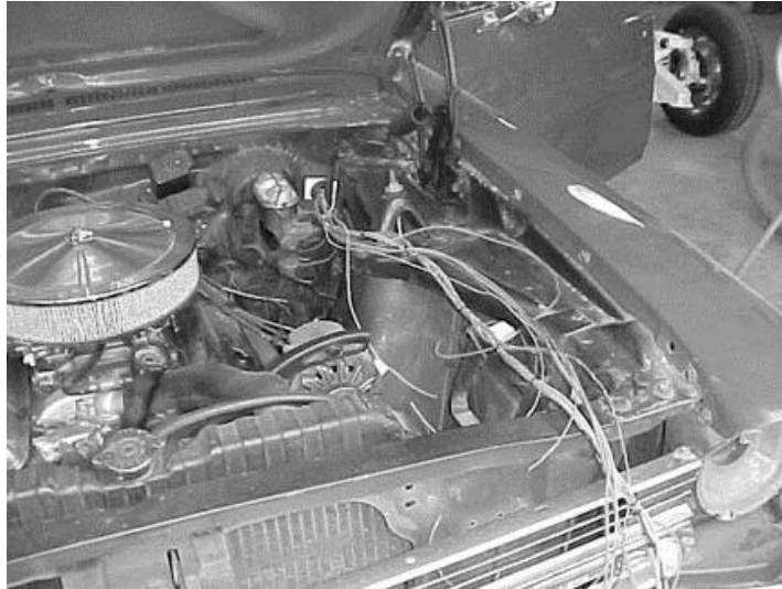
Figure 8.1 Pre-Routing Engine and Headlight Sections
