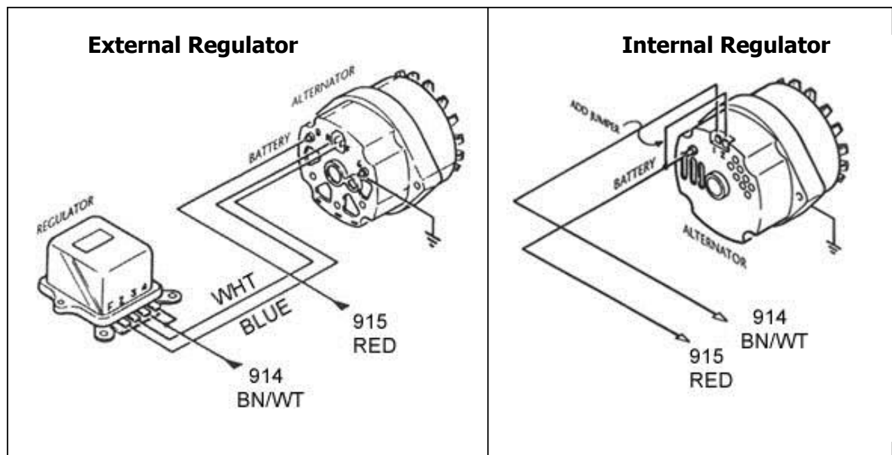
Figure 8.15 Alternator Connections
