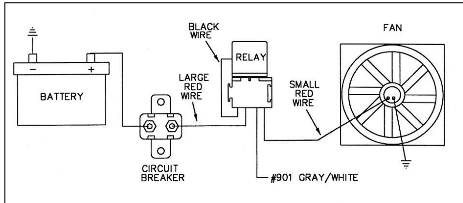
Figure 8.17 Typical Fan Relay Installation ( Painless Part #30101 Fan Relay Kit )
