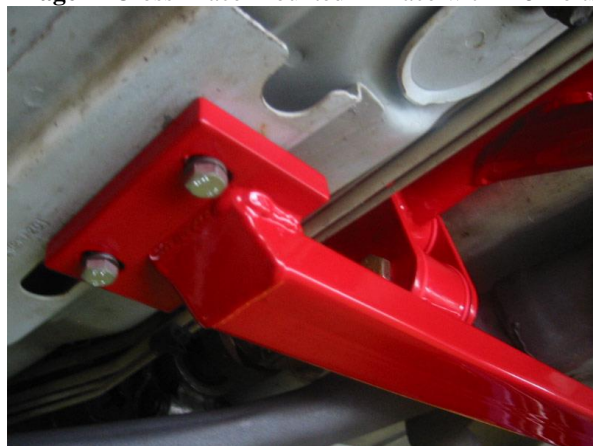
Image 1- Cross Brace Mounted in Place with M8 Bolts
