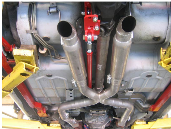
Image 4- Completed Installation with TSP True Duals
