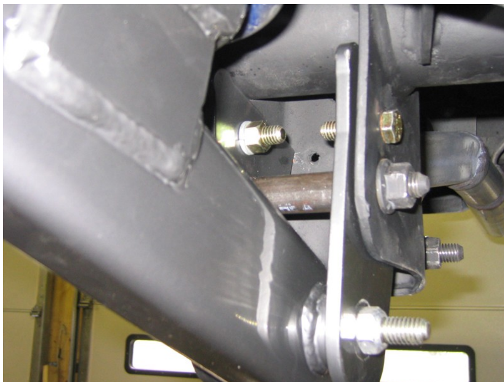
Image 3- Shows (2) holes drilled and 3/8" bolts installed (For bolt-in Applications)
