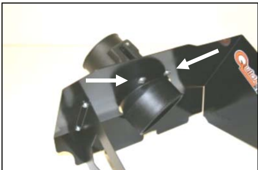
11. Install the MAF adapter (#4) into the Quick Fit Panel using two 1/4"x20 button head bolts (#6) and washers (#7).
