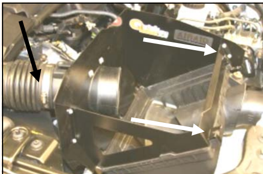
12. Install the MAF adapter into the factory intake tube, and at the same time slide the three tabs on the back of the Quick Fit Panel into the three slots on the factory airbox base. Adjust for fit, then snap the two factory clips to secure the panel. Next tighten the hose clamp where the factory tube slides over the MAF adapter.
