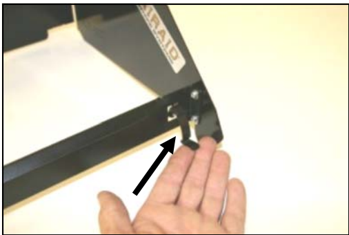
10. Reinstall the factory clip that was removed in step #8 onto the front panel of the Quick Fit Panel as shown.
