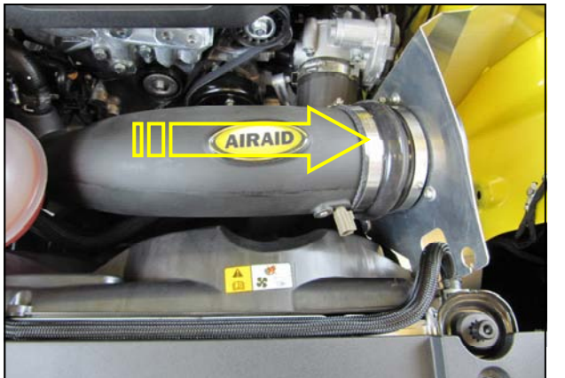
21. Slide the Airaid Intake Tube into the Hump Hose and tighten all four Hose Clamps. Apply the Airaid Bubble Decal onto the Intake Tube as shown.
