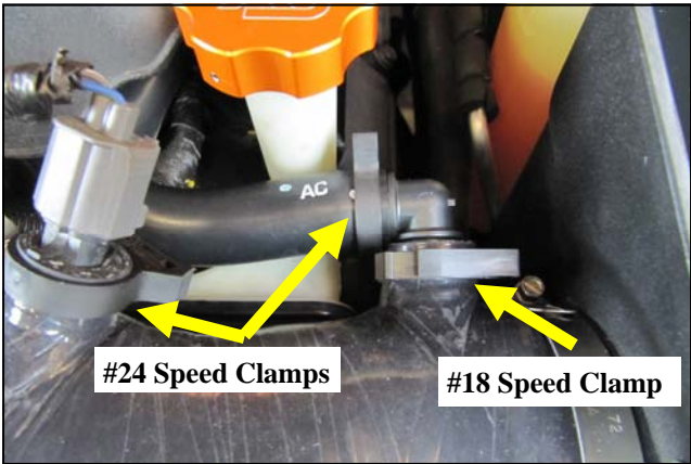
11. Secure the crankspeed breather tube and air temperature sensor using two #24 Speed Clamps. Secure the Barbed Elbow using the #18 Speed Clamp. Tighten the Intake Tube Hose Clamps at this time.
