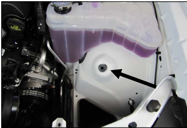
10. Set the Well Nut into the hole in the inner fender.
