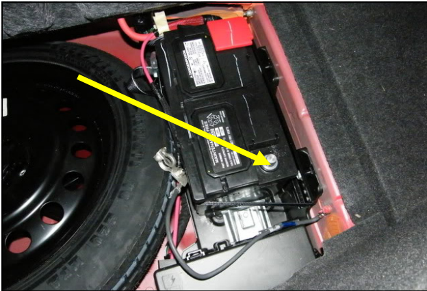
1. Disconnect the negative battery terminal, located in the trunk, by the spare tire.
