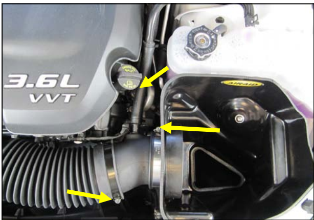
12. Slide the factory intake tube onto the Airaid Tube, adjust if necessary and tighten the Clamps. Connect the crank case breather line to the Barbed fitting using the supplied PCV Hose.
