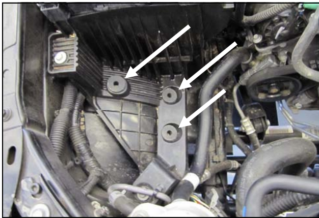
10. Replace the factory airbox grommets in the inner fender area with the three 3/8" Well Nuts.
