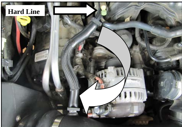
15. Remove the factory breather hose from the hard line, flip it and re connect it back onto the hard line. Connect the opposite end to the Barbed Fitting on the Intake Tube. Secure it using a single Speed Clamp on each end.
