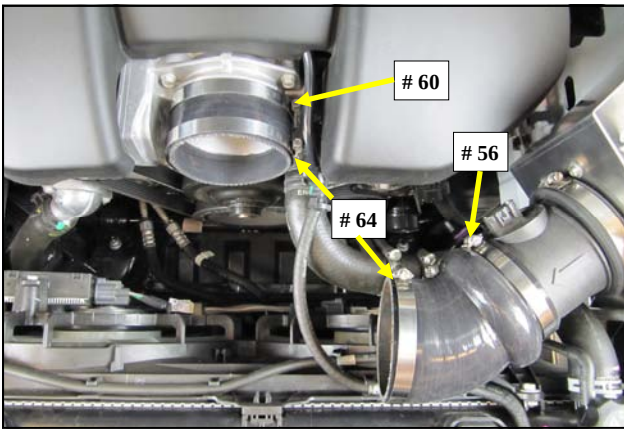
13. Slide the Reducing coupler and #60 clamp onto the throttle body with the #64 clamp on the larger end on the Tube side. Slide the Hump Hose, #56 and 64 Clamps onto the Air meter as shown. Leave the Clamps loose for now.
