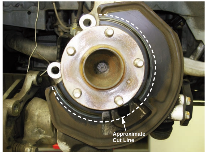
Photo 1. Dust Shield Modification
