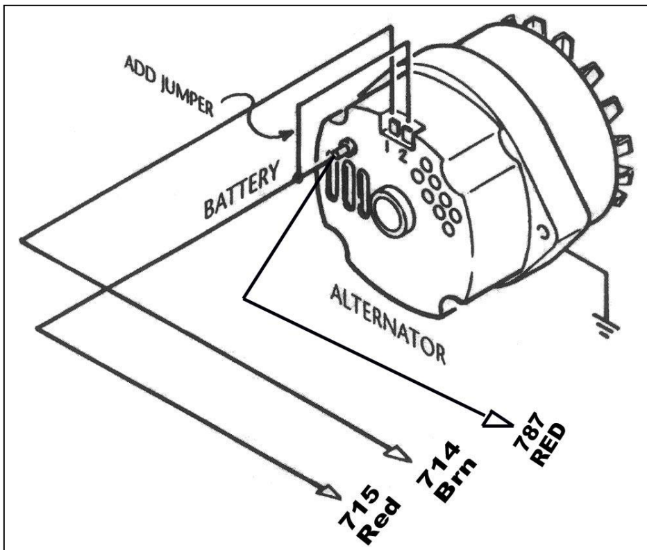
Illustration J Delco Alternator (Internal)
