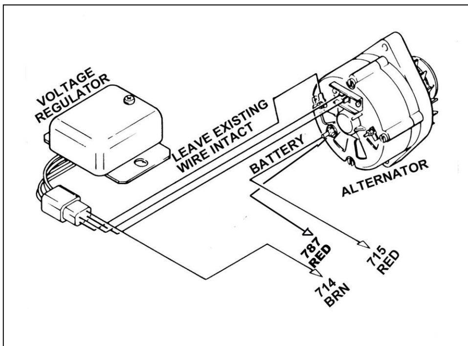
Illustration L Motorola Charging System
