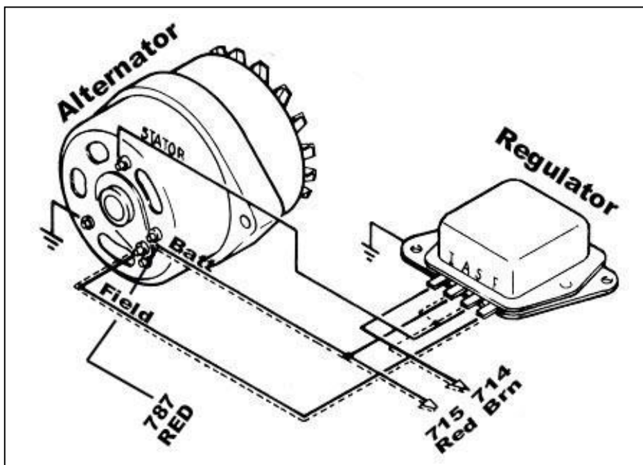
Illustration I Motorcraft Alternator
