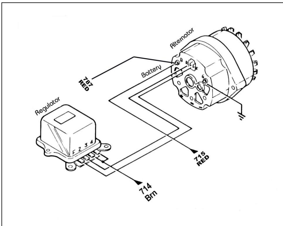
Illustration K Delco Alternator (External)
