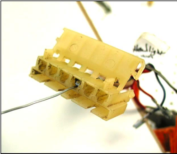
Figure 7.1.2 Headlight Switch Terminal Removal
