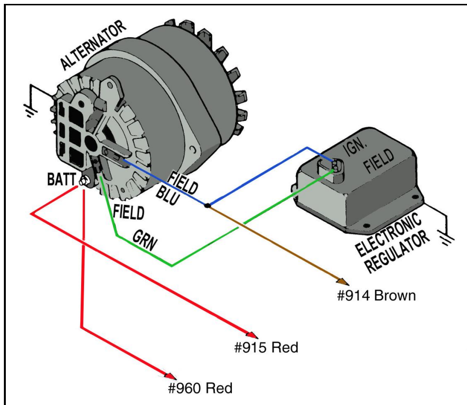
Diagram 11 Mopar Alternator
