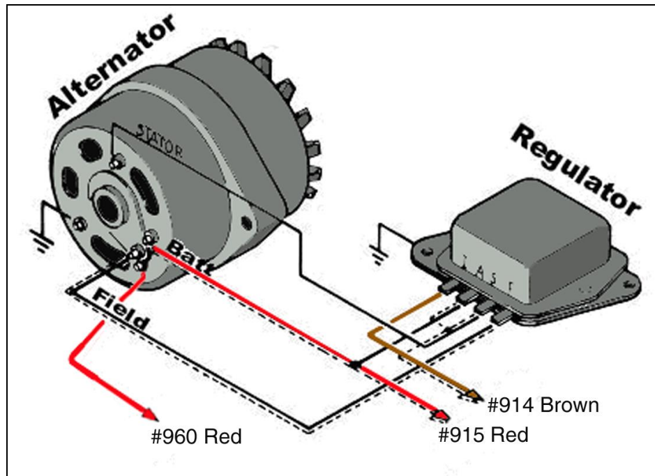
Diagram 12 Motorcraft Alternator
