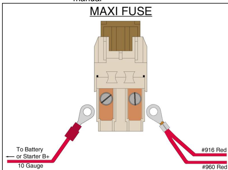
Diagram 8 Maxi Fuse
