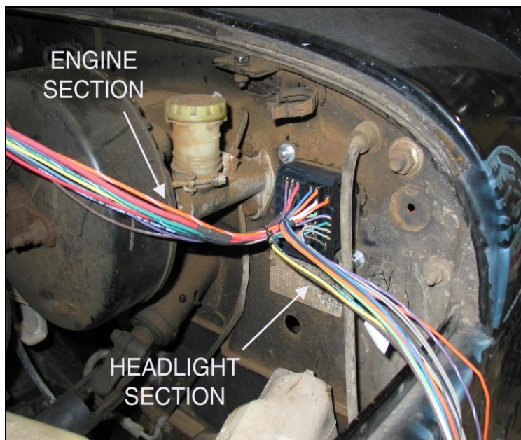
Figure 9.0 Front Harness
