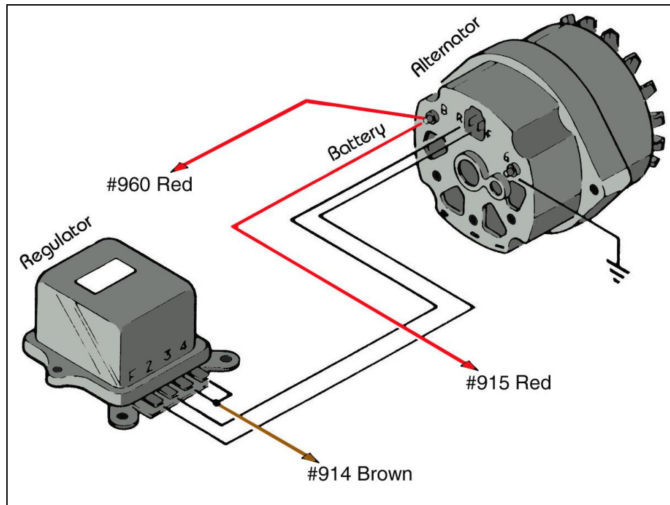
Diagram 10 Delco Alternator
