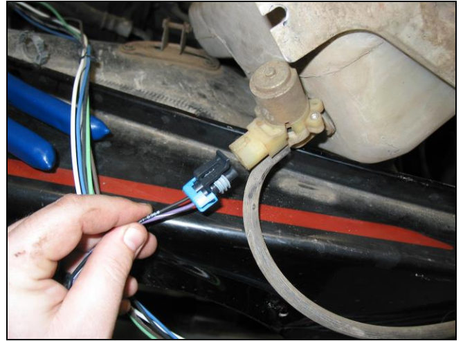
Figure 9.2.2 Washer Pump
