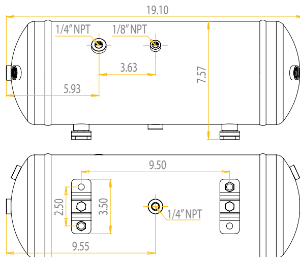
3 Gallon Air Tank
