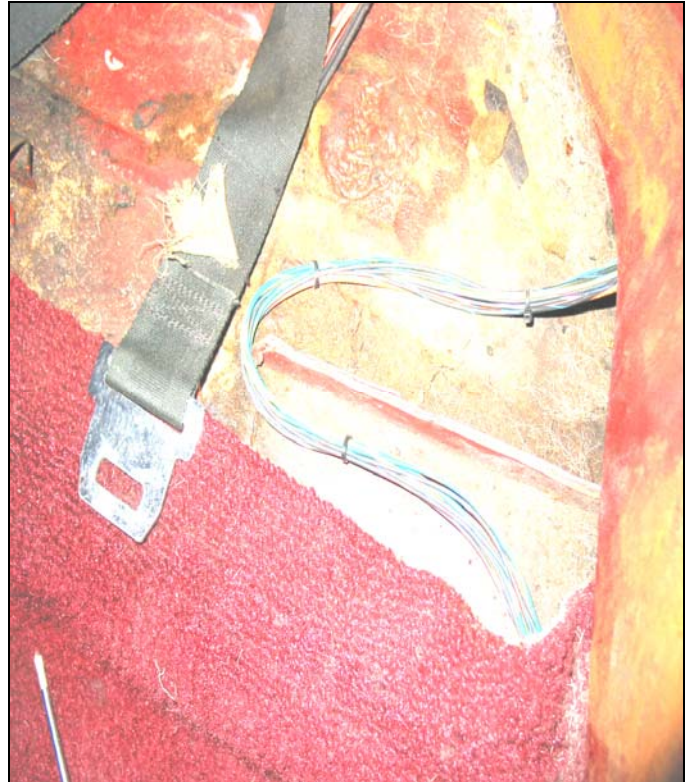
Figure 6-8B Tail Section Routing
