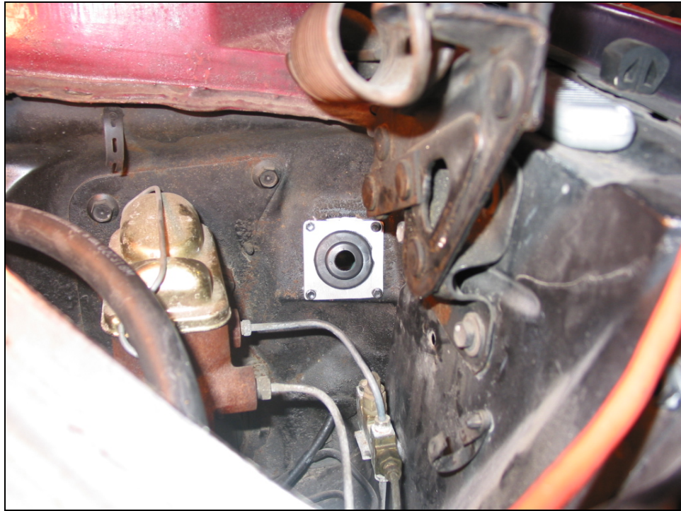
Figure 6-5 Firewall Plate
