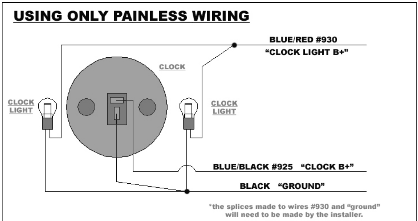
Figure 7-29B Clock Wiring
