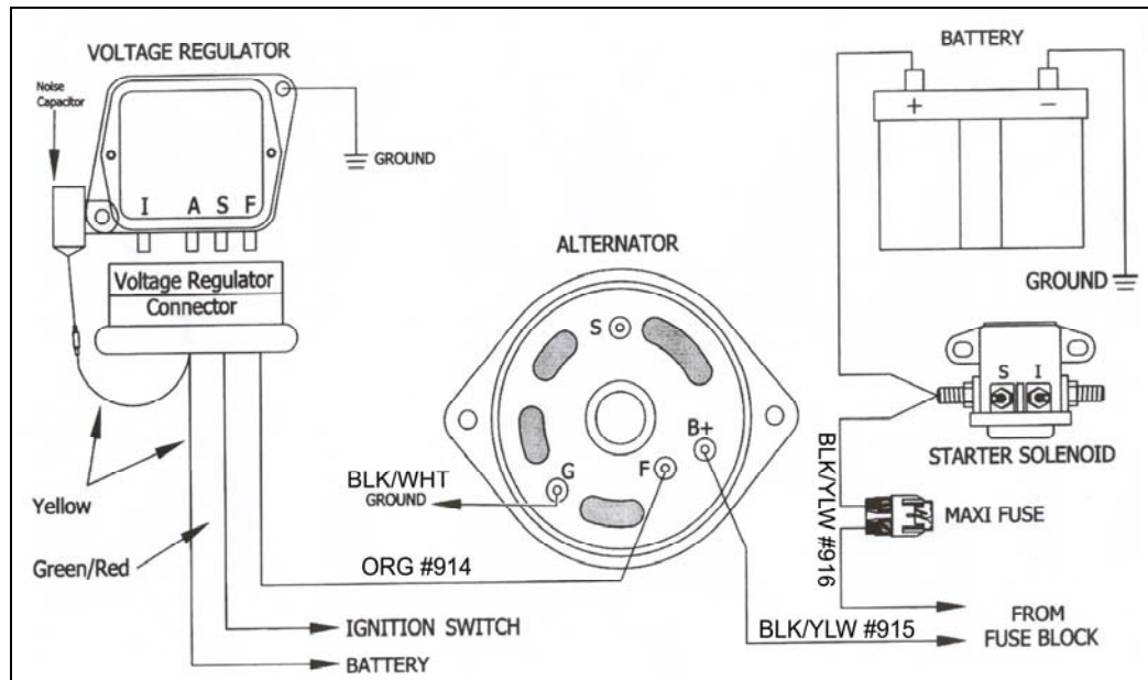
Figure 7-1 Alternator/Regulator Connections
