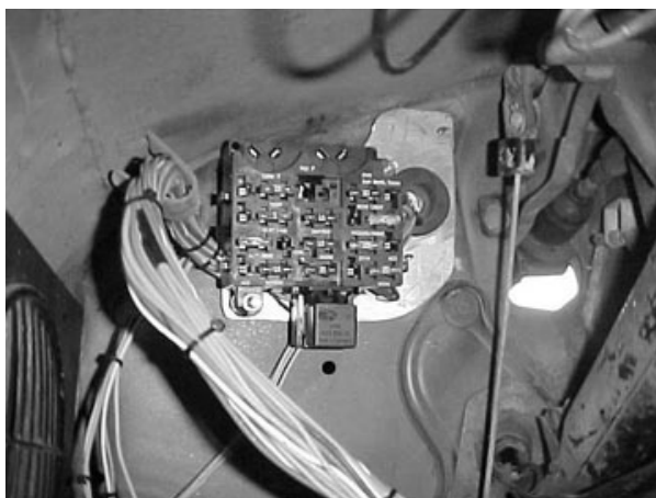
Figure 8.3 Fuseblock Mounted
