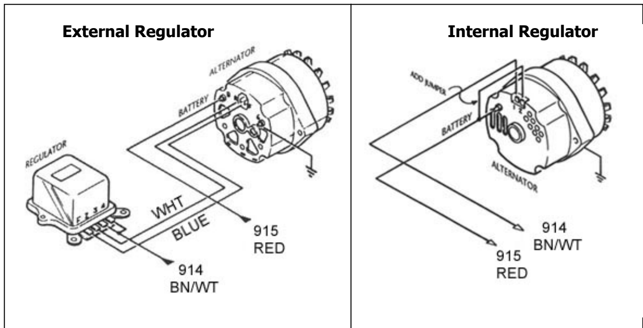
Figure 8.15 Alternator Connections
