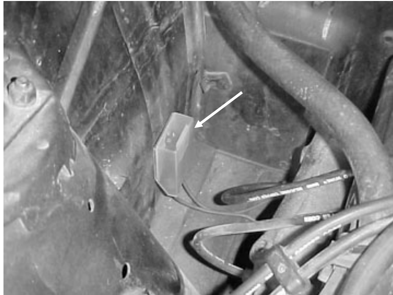
Figure 8.13 Maxi Fuse
