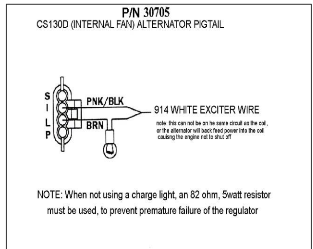
Figure 7-2E CS-130D Connector and Pin Out
