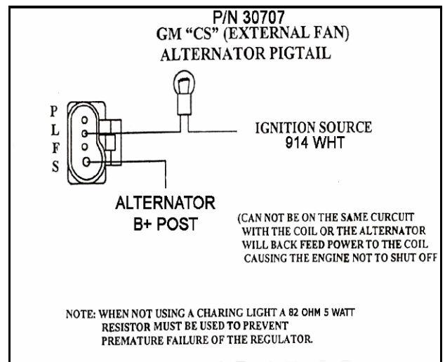
Figure 7-2C CS-130 Connector and Pin Out
