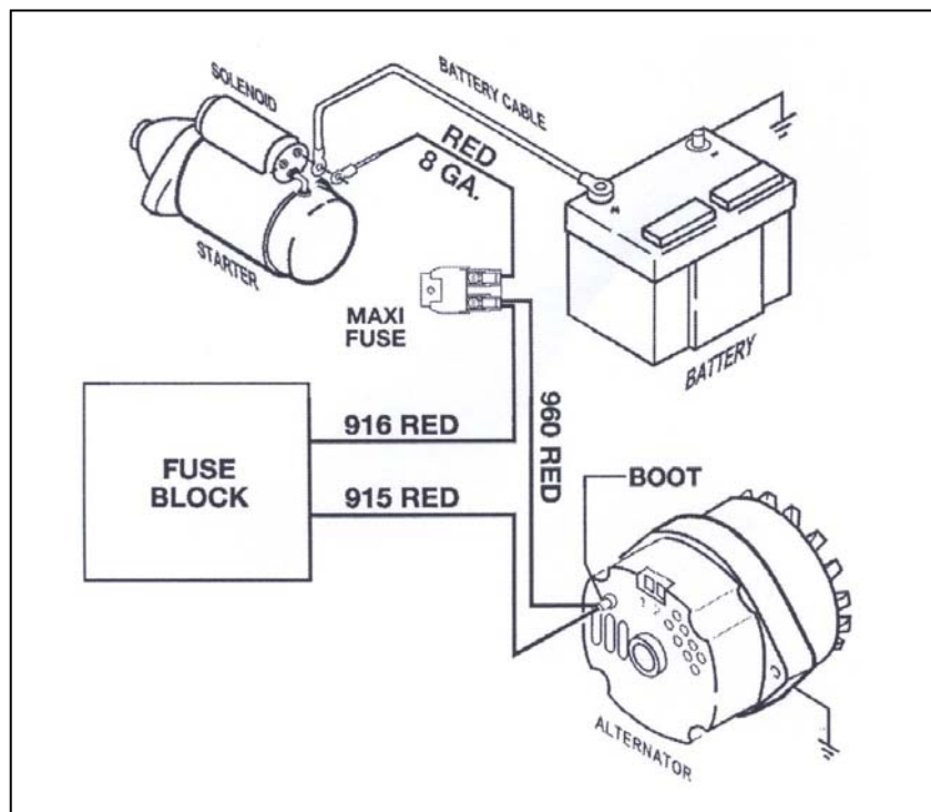
Figure 9-1B High Output Wire
