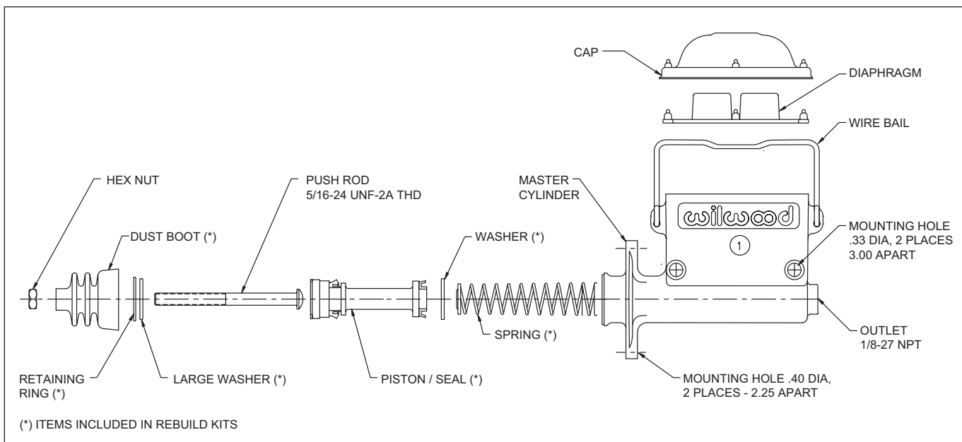
Wilwood High Volume Aluminum Master Cylinder Exploded Diagram
